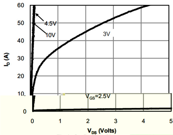
Figure 1: DC Power Characteristics
