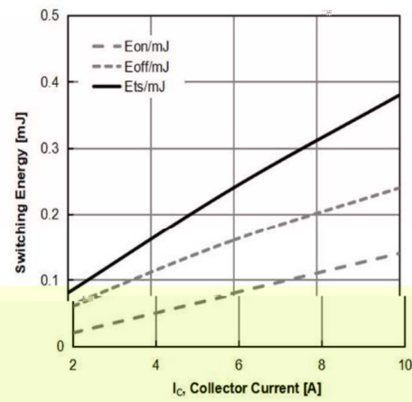
Fig14. TYP. Switching Energy vs. Collector Current (TJ=25°C, VCE=400V, VGE=15V, Rg=5Ω)
