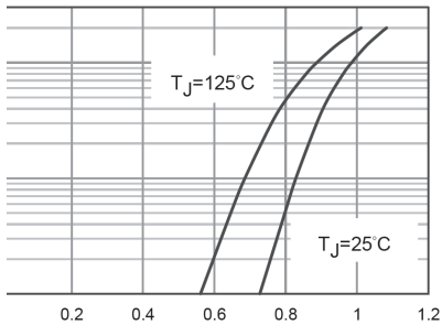
G.4-TYPICAL FORWARD CHARACTERISTICS
